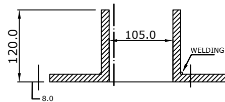
SPINDLE PLATE
