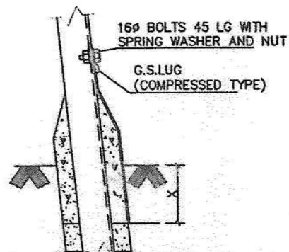
LUG FITTING FOR THREE LEGS (TYPICAL)
