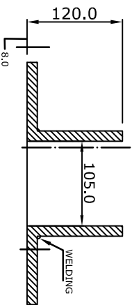
SPINDLE PLATE
